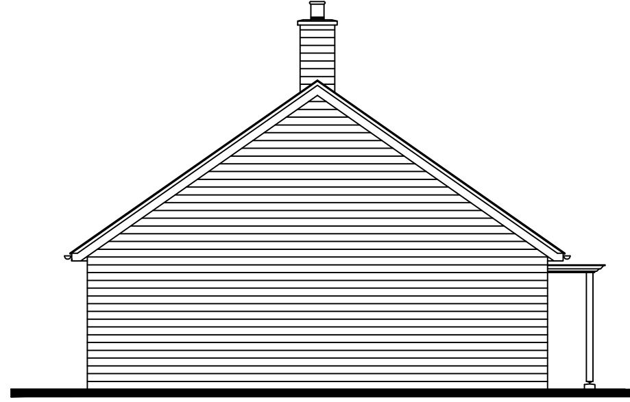
SIDE ELEVATION
