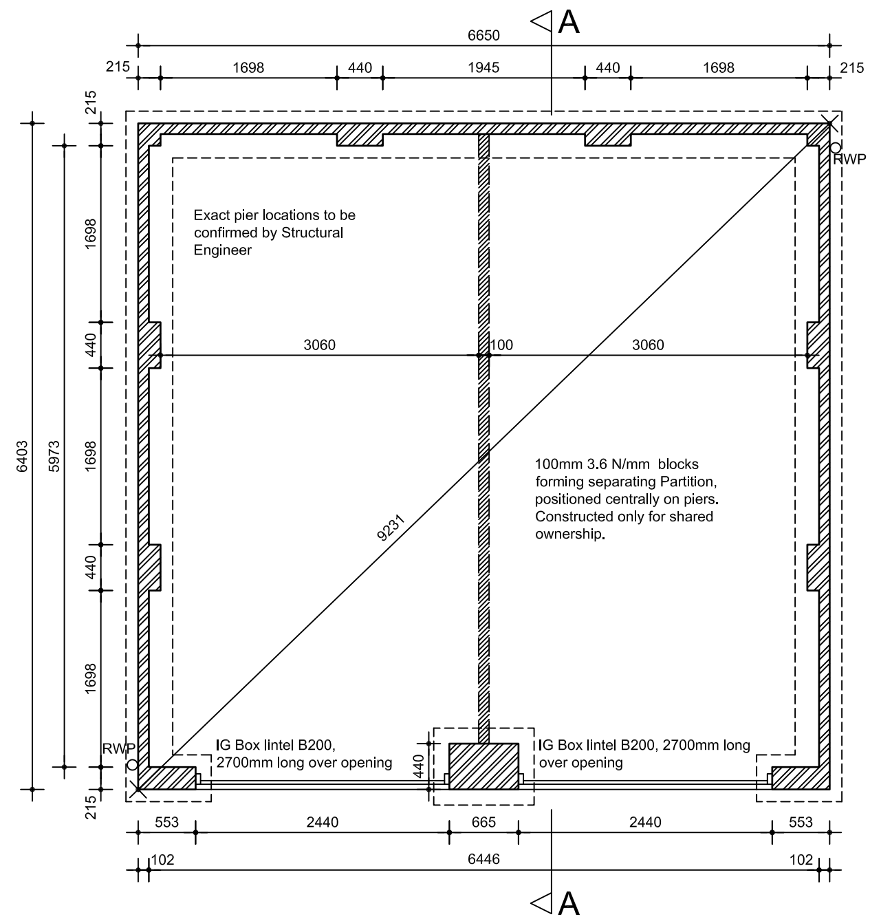
Floor Plan
